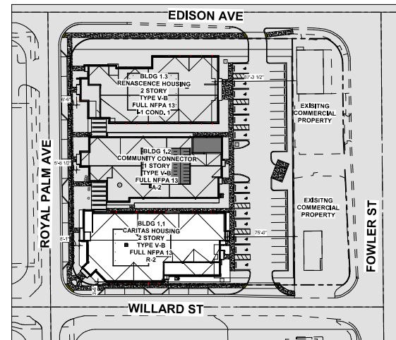
③ BDLG 1.1 - ARCHITECTURAL SITE 1" = 40'-0"
